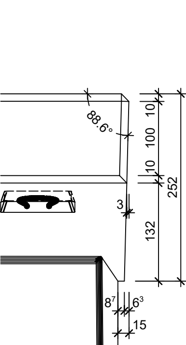
Detail A, 1:5
