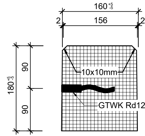
Detail 1, 1:5
