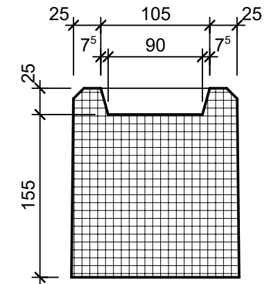
Detail 2, 1:5
