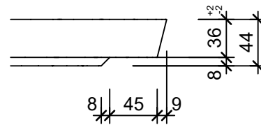
Detail A, 1:5
