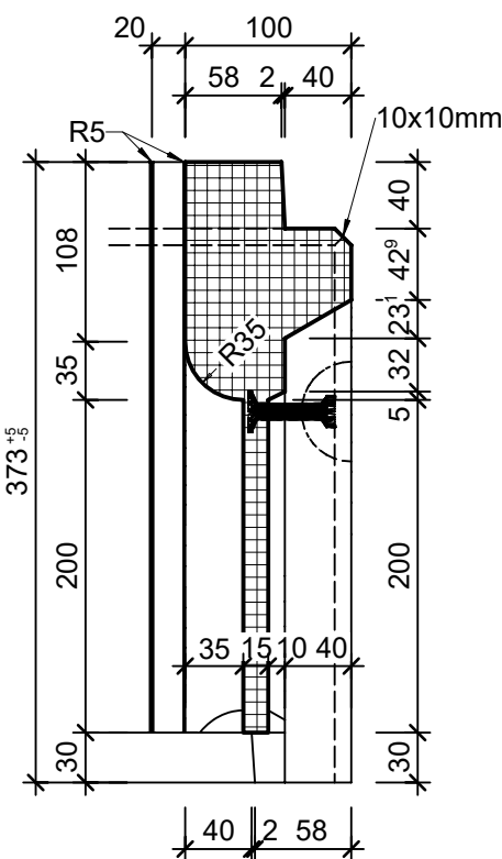
Detail A, 1:5
