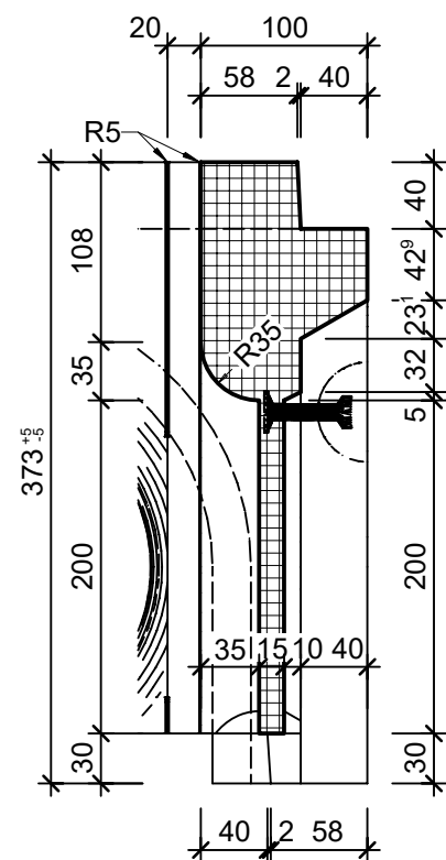
Detail A, 1:5
