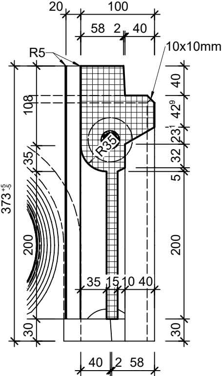
Detail A, 1:5
