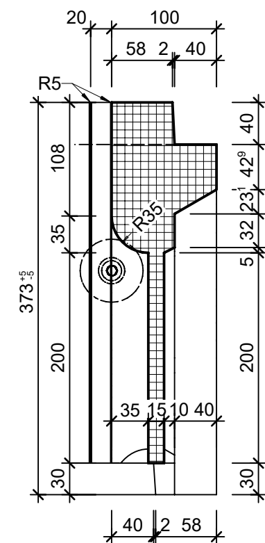
Detail A, 1:5
