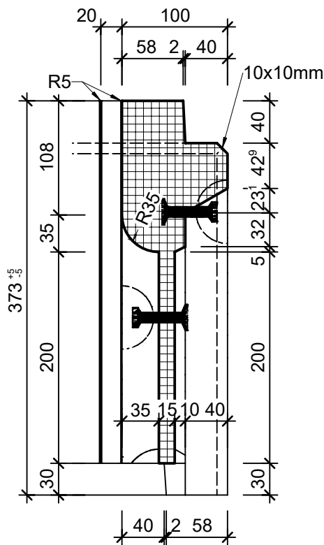
Detail A, 1:5
