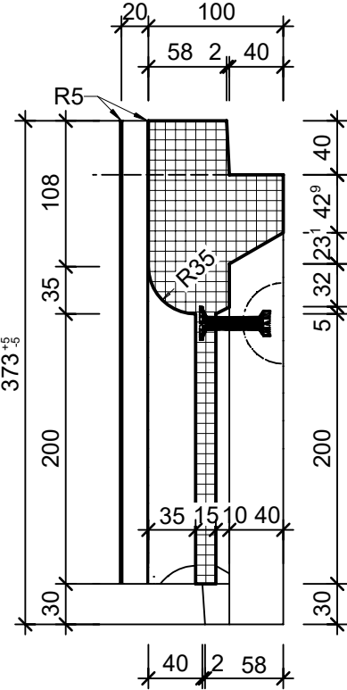
Detail A, 1:5
