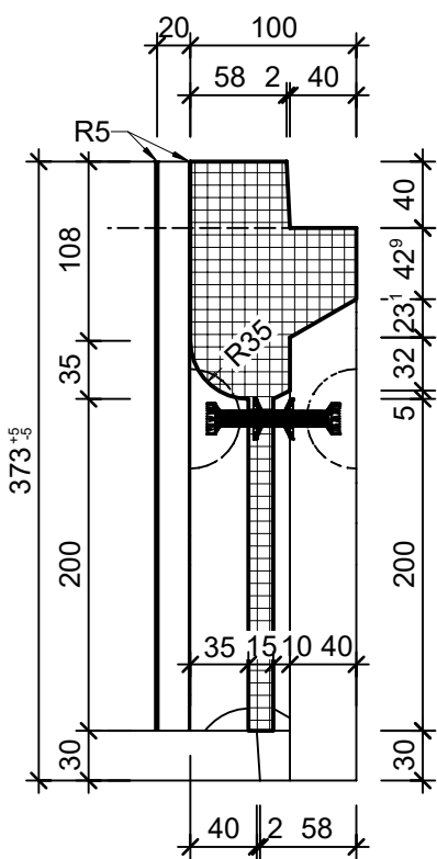
Detail A, 1:5
