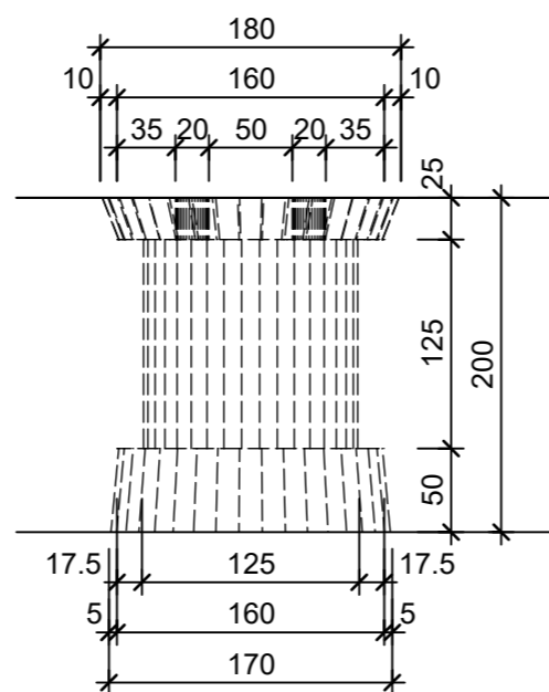
Detail A, 1:5
