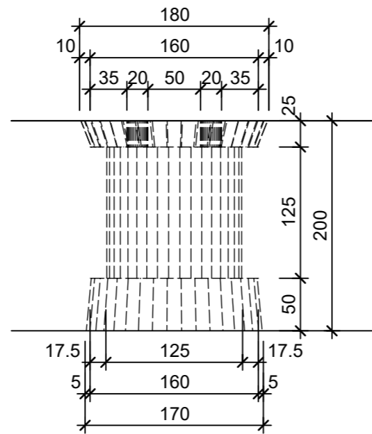
Detail A, 1:5
