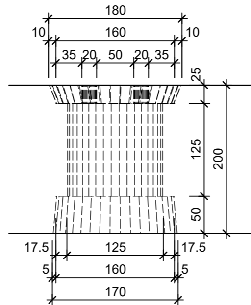
Detail A, 1:5
