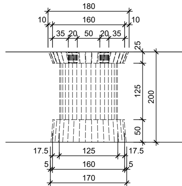
Detail A, 1:5
