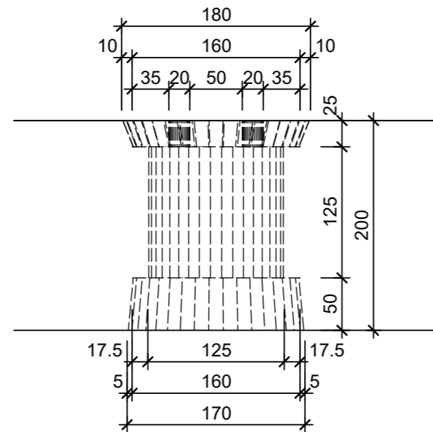
Detail A, 1:5
