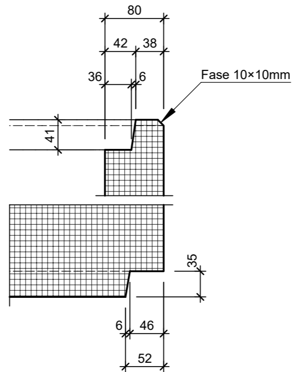
Detail 1, 1:5
