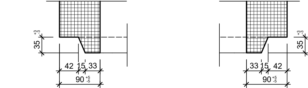
Detail B, 1:5
