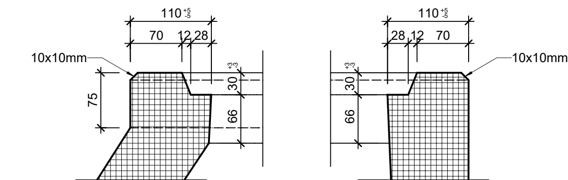
Detail B, 1:5
