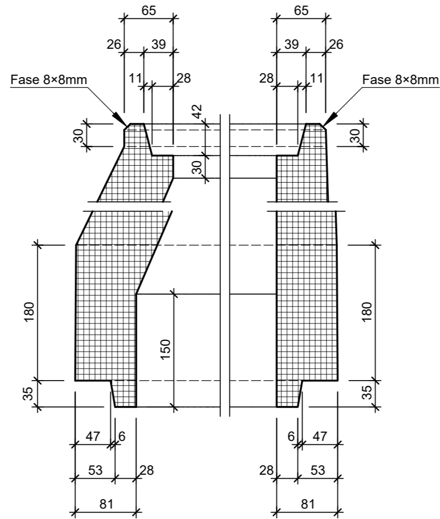
Detail 1, 1:5
