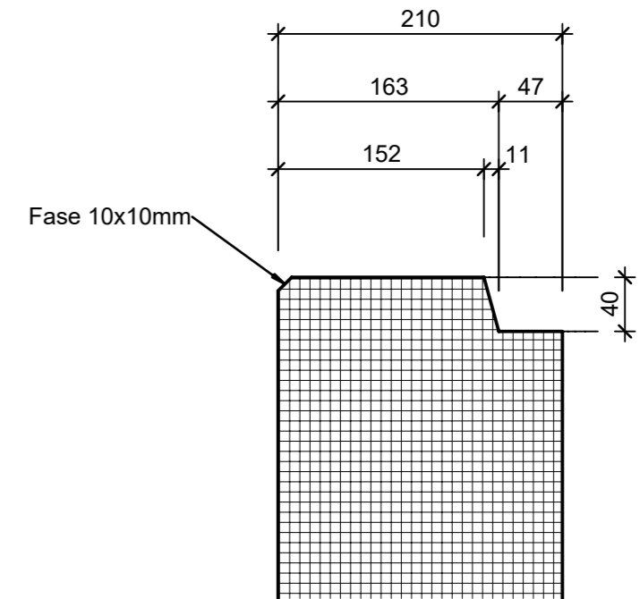
Zapfendetail, 1:5
