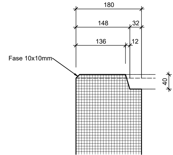
Zapfendetail, 1:5
