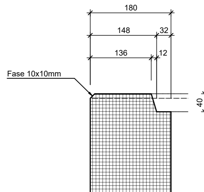
Zapfendetail, 1:5
