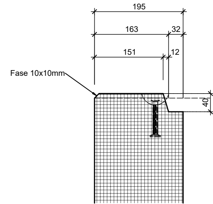
Zapfendetail, 1:5
