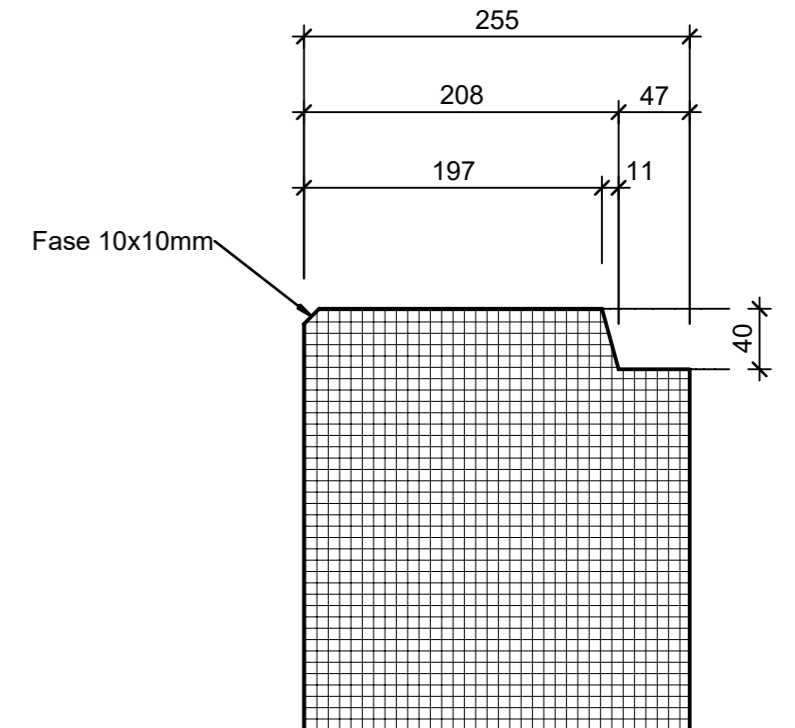
Zapfendetail, 1:5
