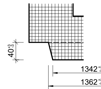
Detail Spitzende, 1:5
