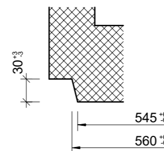
Detail Spitzende, 1:5
