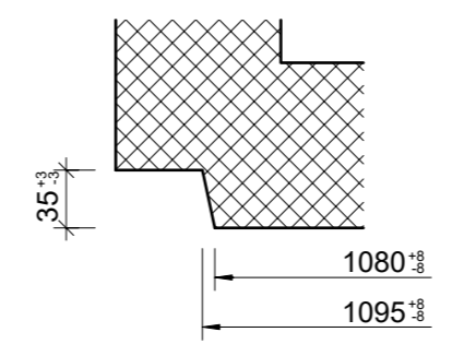
Detail Spitzende, 1:5
