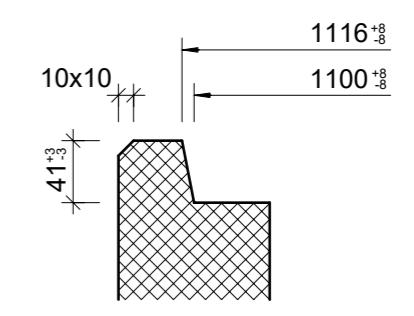
Detail Muffe, 1:5
