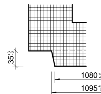
Detail Spitzende, 1:5
