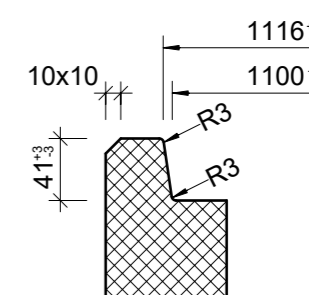
Detail Muffe, 1:5
