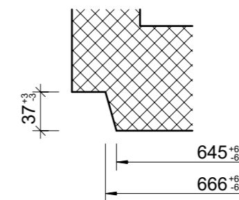
Detail Spitzende, 1:5
