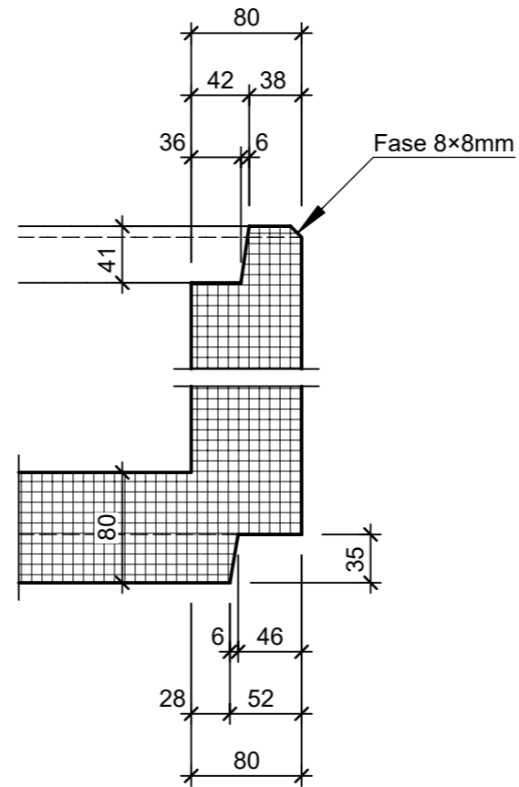
Detail 1, 1:5
