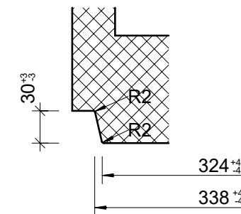
Detail Spitzende, 1:5
