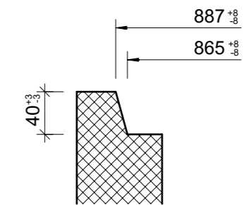
Detail Muffe, 1:5
