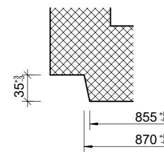
Detail Spitzende, 1:5
