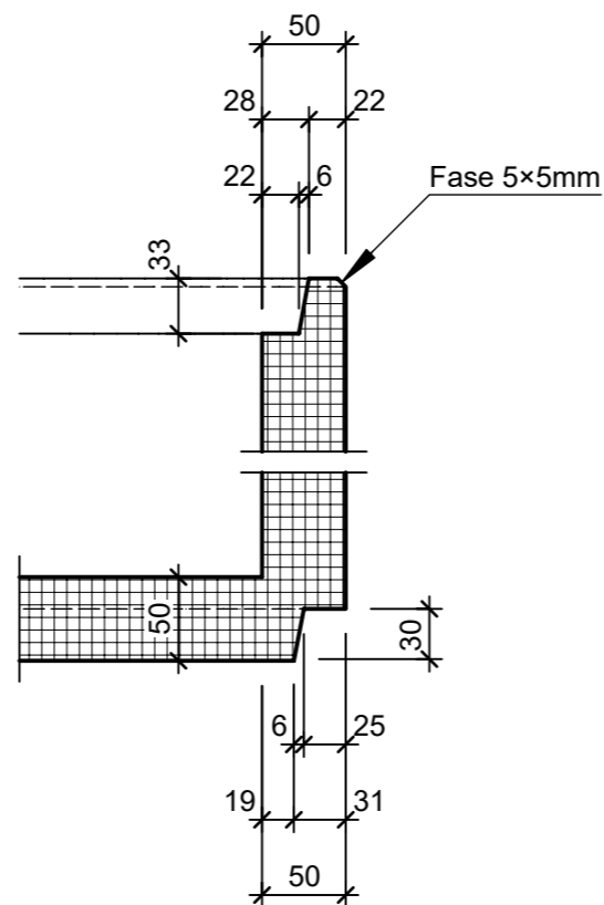
Detail 1, 1:5
