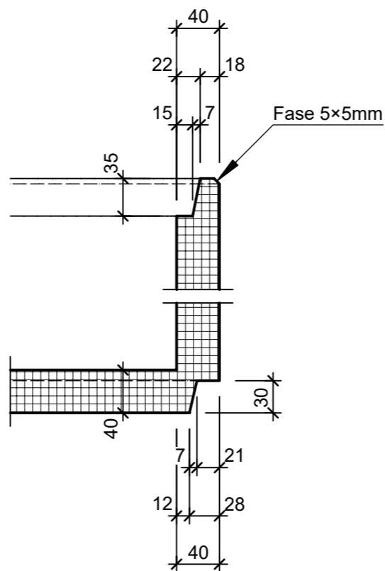
Detail 1, 1:5
