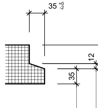
Detail B, 1:5
