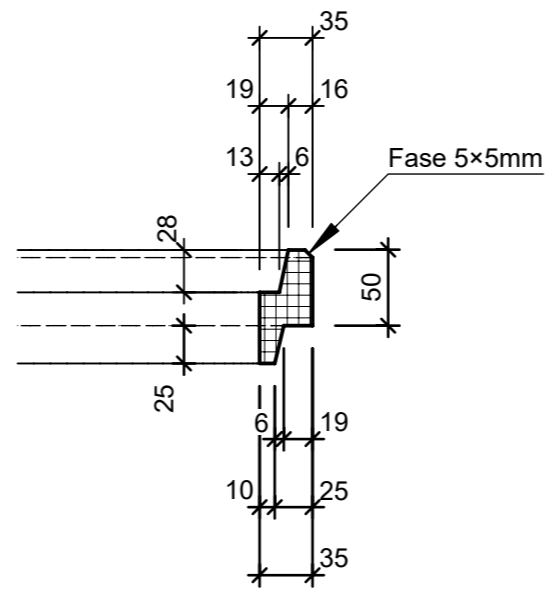
Detail 1, 1:5
