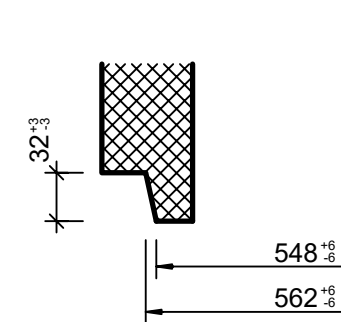
Detail Spitzende, 1:5
