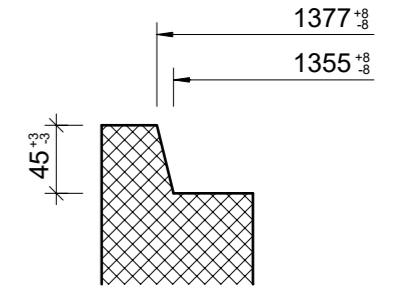
Detail Muffe, 1:5
