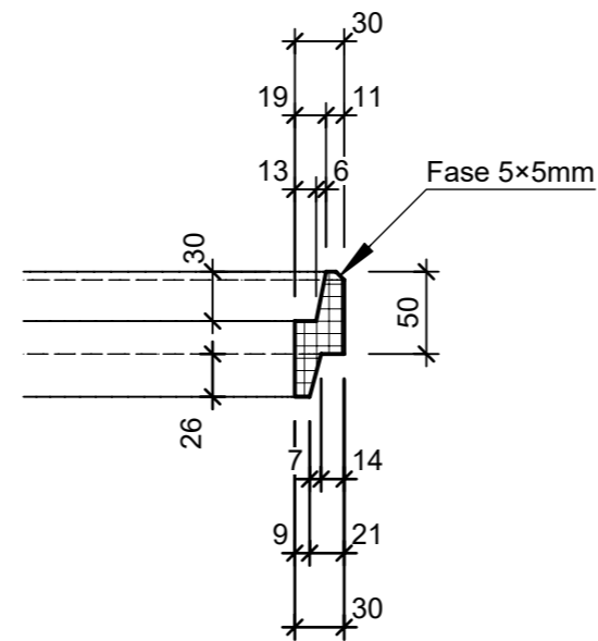
Detail 1, 1:5
