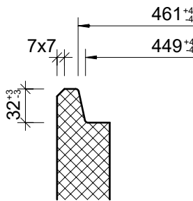
Detail Muffe, 1:5
