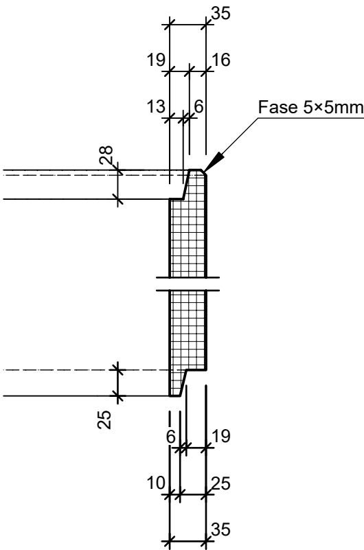
Detail 1, 1:5
