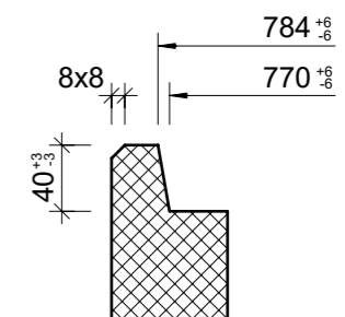
Detail Muffe, 1:5
