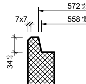
Detail Muffe, 1:5
