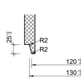
Detail Spitzende, 1:5
