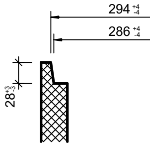
Detail Muffe, 1:5
