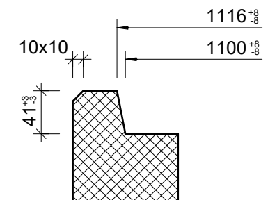
Detail Muffe, 1:5
