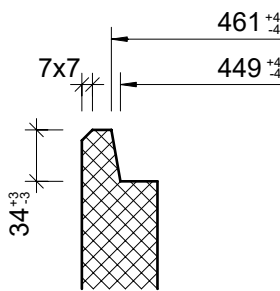
Detail Muffe, 1:5
