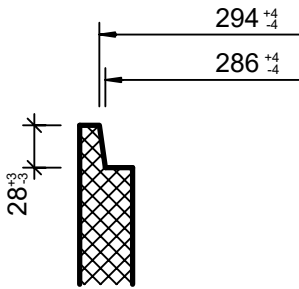
Detail Muffe, 1:5
