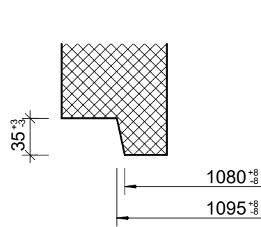
Detail Spitzende, 1:5
