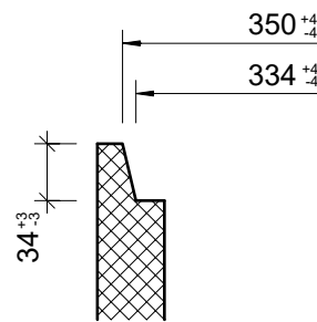
Detail Muffe, 1:5
