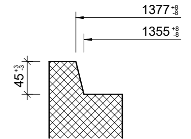
Detail Muffe, 1:5
