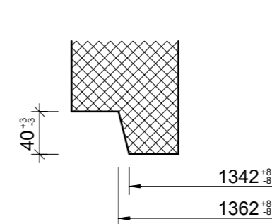
Detail Spitzende, 1:5
